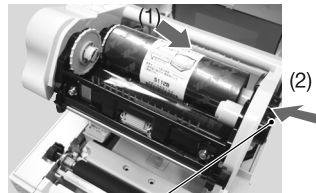
Ribbon supply unit core guide
